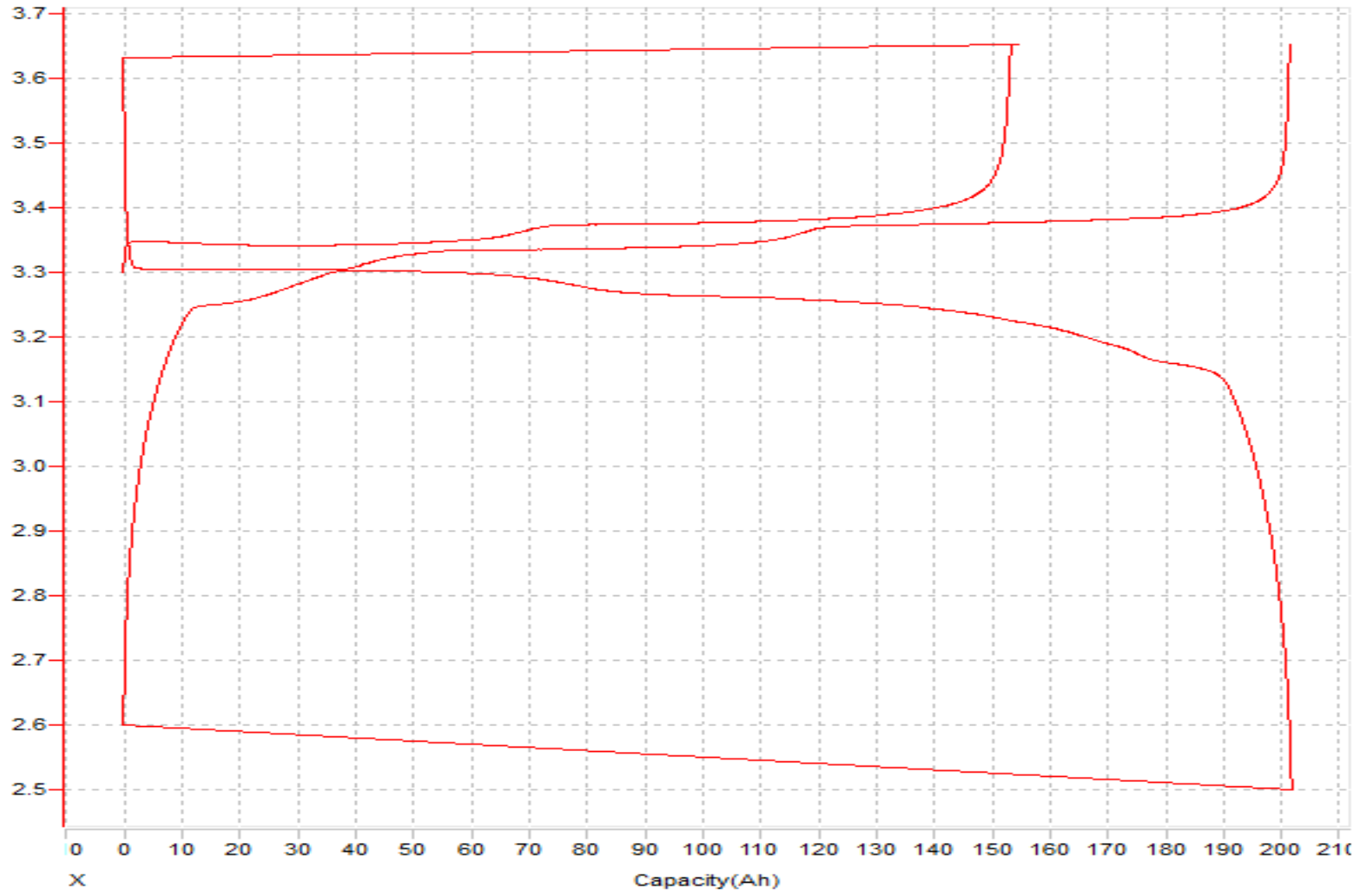
Capacity--Voltage
