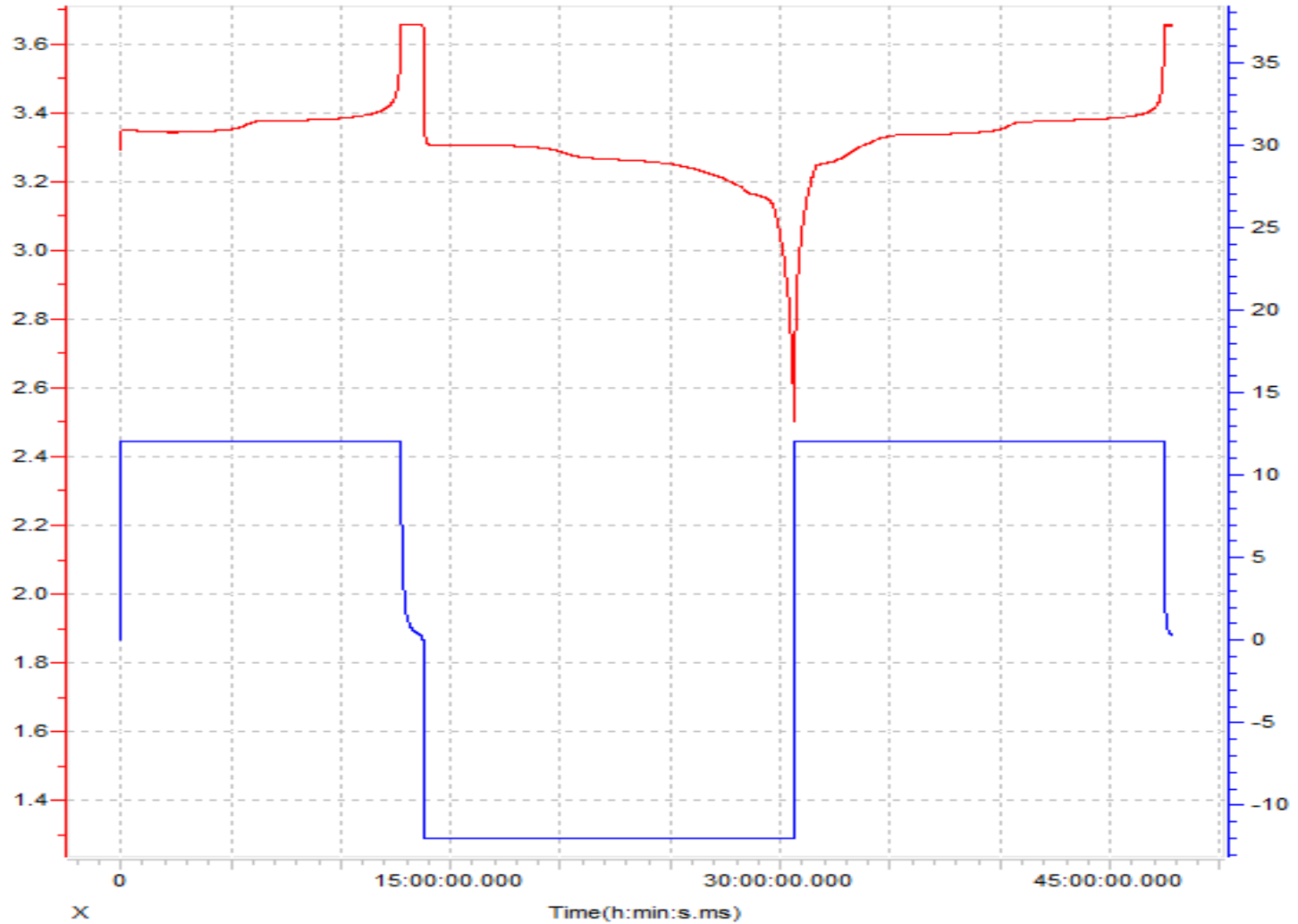
Time--Voltage&&Current
